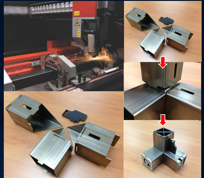
Pipe Laser Cutting
